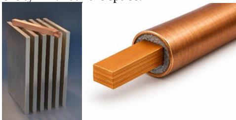
Fig. 1: HTS composite conductor atop a 20 kA aluminum busbar (left) and visualized cross-section (right).
